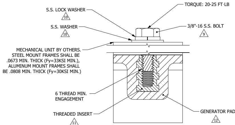
2 ANCHOR DETAIL 2:3 SCALE SECTION VIEW
