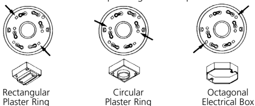
FIGURE 5 SELECT CORRECT MOUNTING HOLES ON TRIM RING
