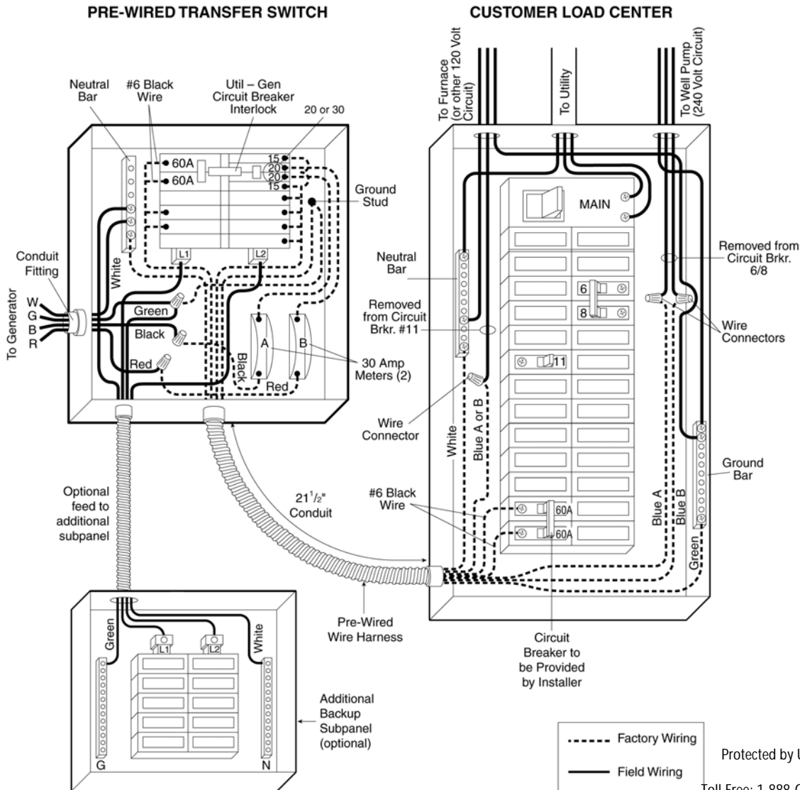
Figure 2 - WIRING DIAGRAM:
