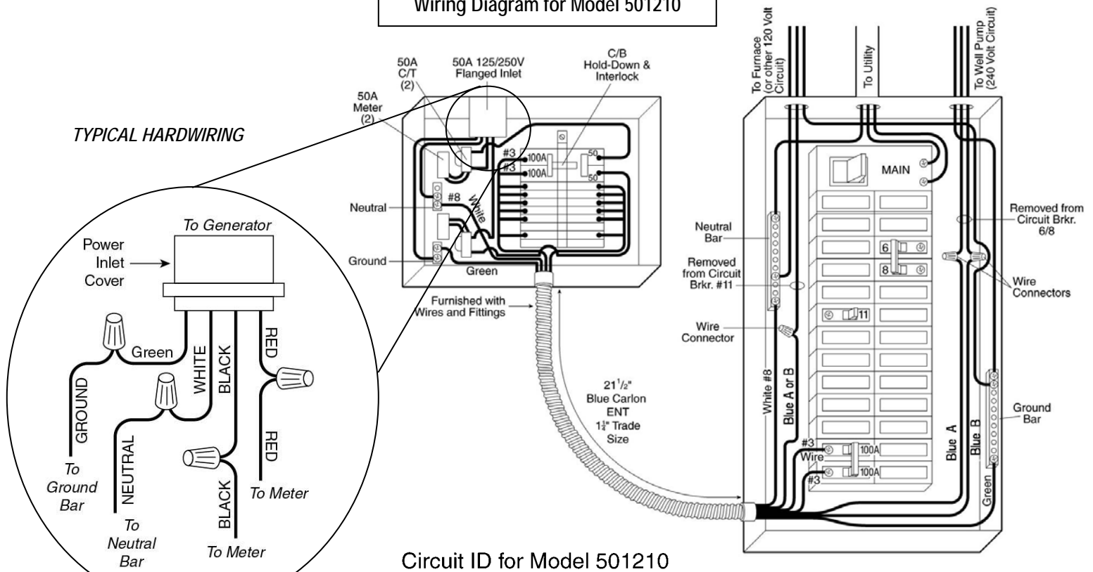
Wiring Diagram for Model 501210
