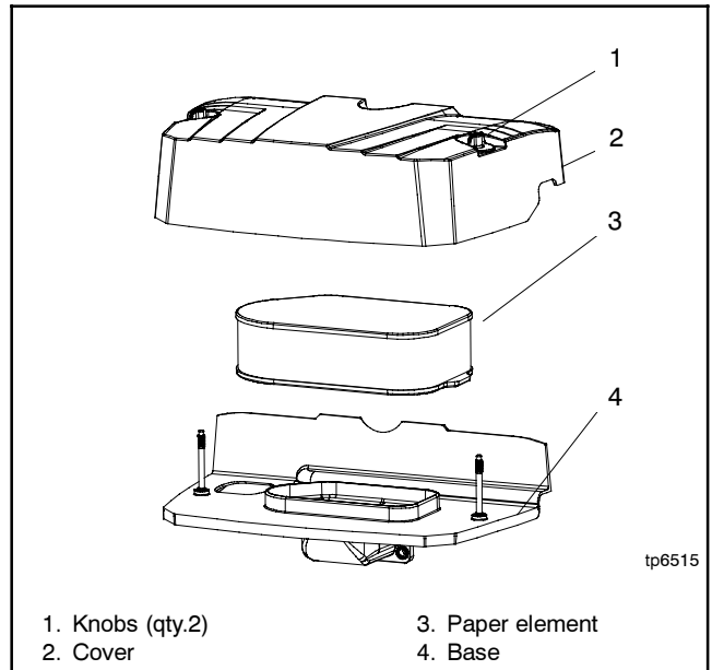
Figure 6 Air Cleaner, 17/18/20 kW
