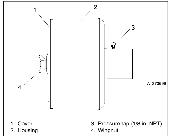
Figure 8 Air Cleaner, 48 kW
