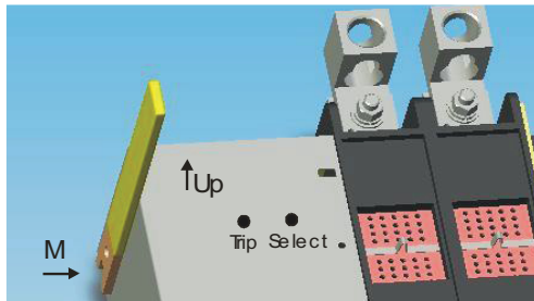
Figure 10 – Manual Transfer Lever Location
