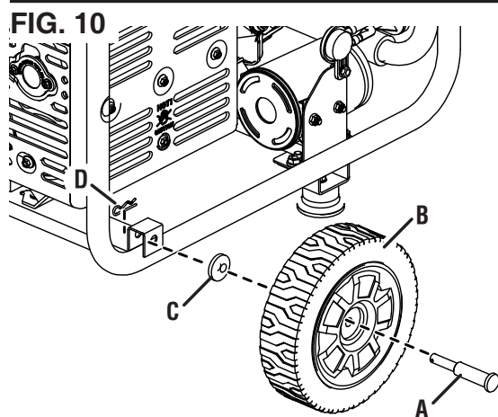
A - Axle B - Wheel C - Washer D - Hitch Pin
