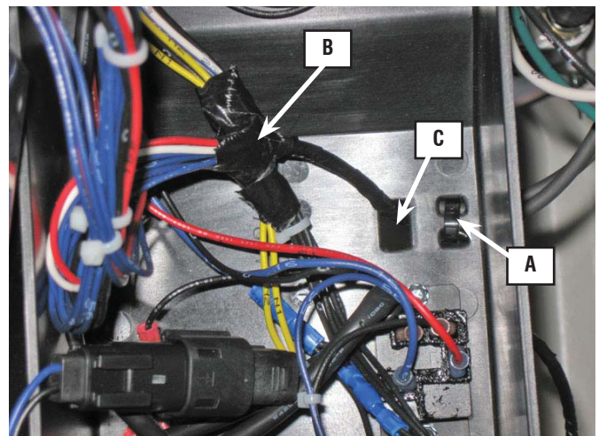
Figure 2 — 4-wire LED Wire Harness Position
