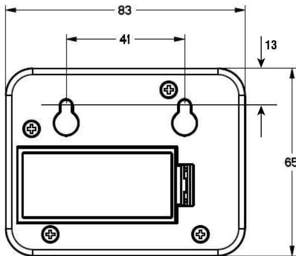
Figure 13 – Mounting hole locations
