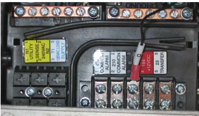
Figure 8 – Connect the 0 Wire
