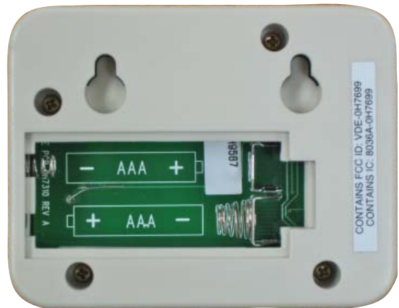
Figure 9 – Battery installation
